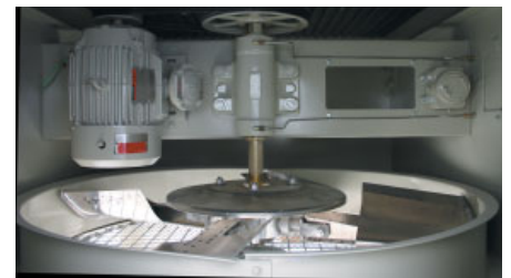
Plenum-Mounted Electric Drive on Model HR (Standard)
